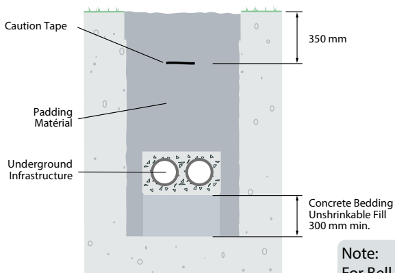
Figure 10 - Concrete Underground Infrastructure
