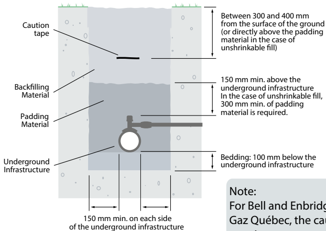
Figure 9 - Non-Concrete Underground Infrastructure
