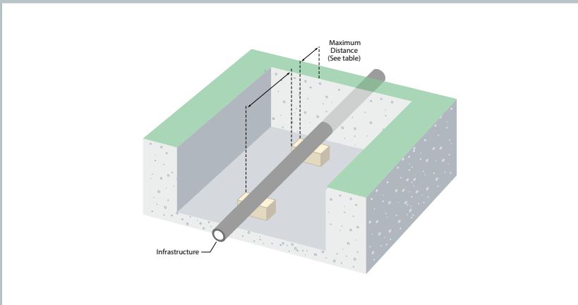
Figure 8 - Underlying Support (Exemple for Énergir et Enbridge Gaz Québec).
